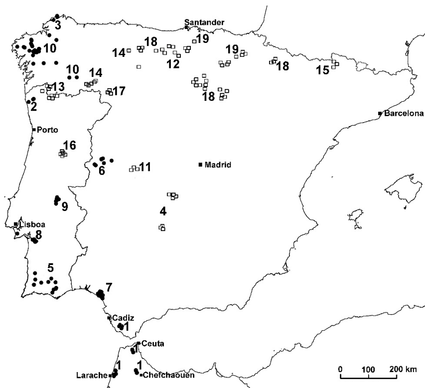
Figure 2. Location of the communities and relevés, used for the cluster analysis. Circles communities belonging to the Ulici lusitanici-Genistion ancistrocarpae, squares to the Genistion micrantho-anglica (community numbers and names see legend to Figure 1).
