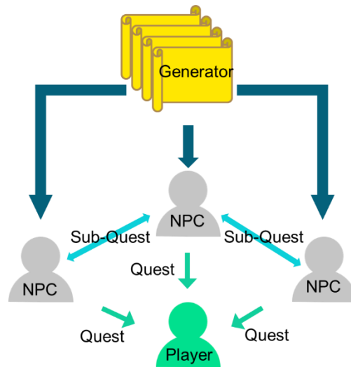
Figure 7. Proposed architecture.
