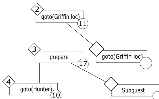
Figure 3. Expansions of <goto> (rule number 11) and <prepare> (rule number 17), both newly added.
