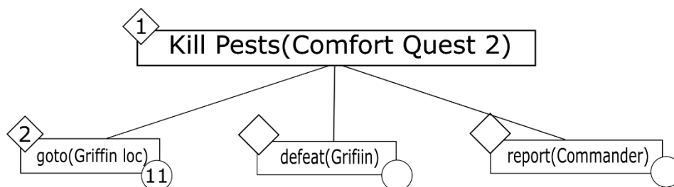
Figure 2. Initial strategy of example quest.
