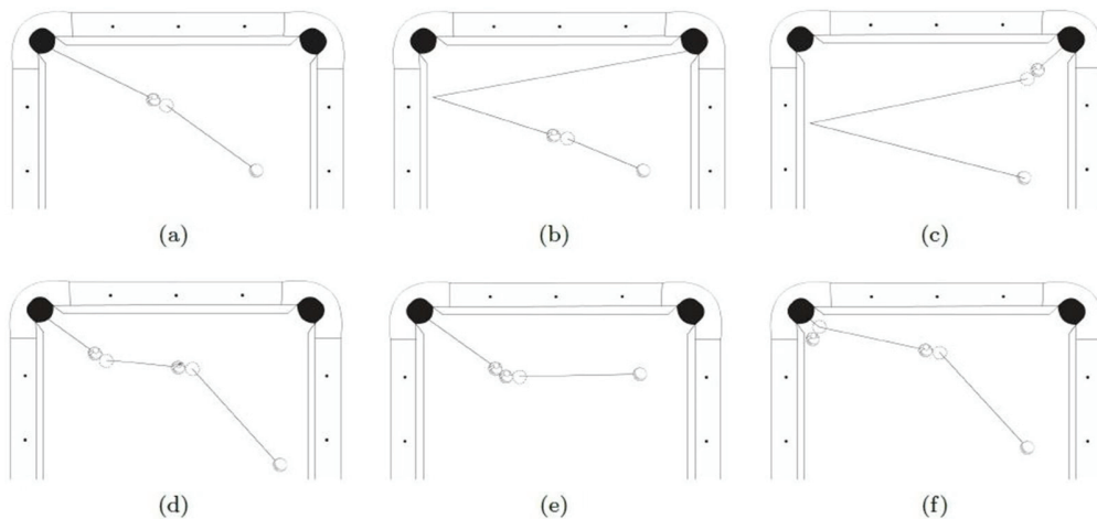
Figure 3. Shot types: (a) direct shot, (b) bank shot, (c) kick shot, (d) combination shot, (e) pulk shot, (f) kiss shot [Bahr, 2012]
