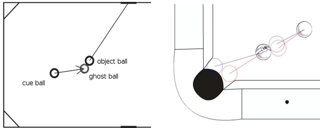
(a) Ghost ball concept [Smith, 2006]
