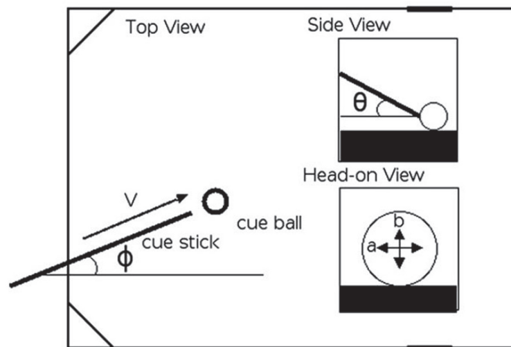
Figure 2. Parameters that define a shot in Billiards [Smith, 2006]
