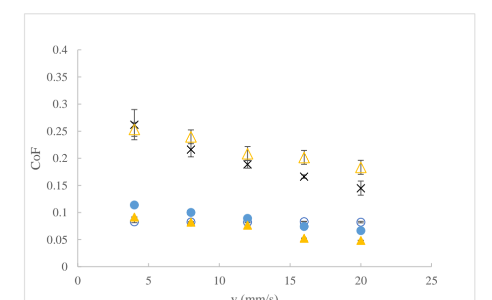
Figure 4: Plots of (CoF) as a function of velocity (v), using force 15mN: ×PEG; ×IL5:PEG; ×IL6:PEG; ×IL5:PEG; ×IL6:PEG.
