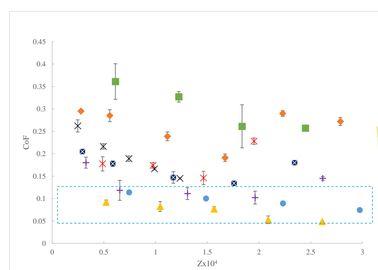
Figure 3: Plots of the friction coefficient (CoF) as a function of the Sommerfeld parameter, (Z=ηv/F), obtained with steel spheres sliding on silicon substrates using force 15mN and velocities between 4 and 20 m/s: ×PEG; ×IL1:PEG; ×IL2:Sulfolane; ×IL2:PEG; ×IL3:PEG; ×IL4:PEG; ×IL5:PEG; ×IL6:PEG. The error bars correspond to standard deviations (n ≥ 4).
