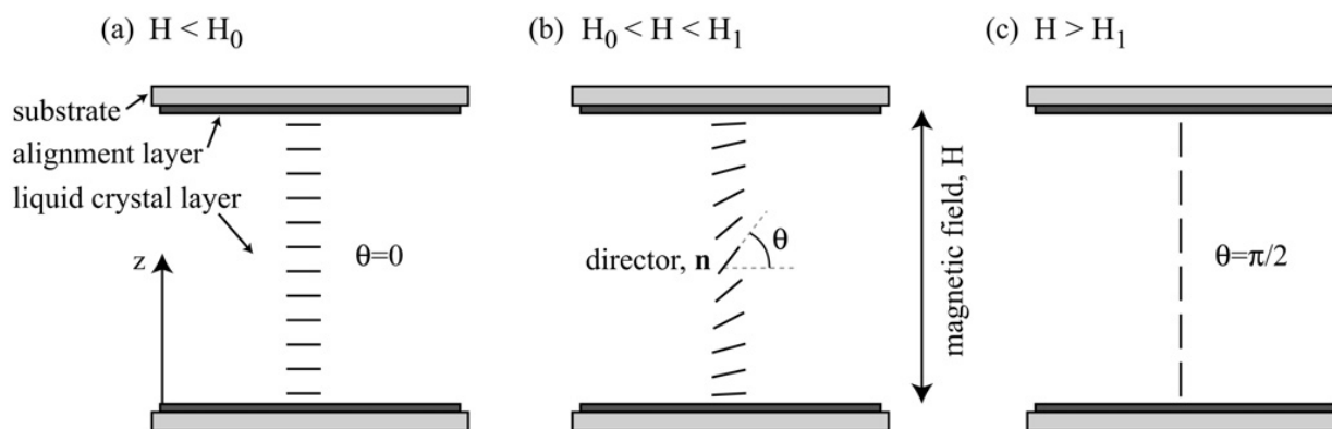
Fig. 1. The Freedericksz cell: (a) With an applied magnetic field below the first critical value, H < H_0 , the liquid crystal director is governed by the preferred alignment layer direction (the x direction). (b) With an applied field H_0 < H < H_1 , the director attempts to reorient to align with the field direction. (c) With a field strength greater than the second critical value, H > H_1 , the director reorients throughout the layer to align with the field direction.
