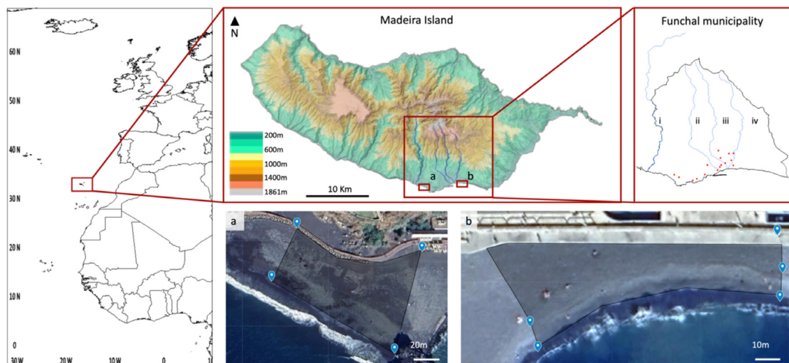
Fig. 1. Location of the study site: Madeira archipelago on the Northeast Atlantic (left), topographic map of Madeira Island denoting the streams and surveyed beaches (top center), and Funchal municipality with the streams (i – Socorridos, ii – São João, iii – Santa Luzia, and iv – João Gomes) that are available in the area (top right). Data from Antunes (2015). Location of the majority of the ATMs (marked with a red dot - top right; number of ATMs in the area as an indicator of the high population density) and aerial views of (a) 'Formosa' and (b) 'Almirante Reis' beaches and respective surveyed areas (down). Source: ATMs locations and images from Google Maps.
