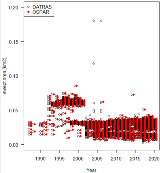
Figure 5.2. Comparison of swept-area estimates in the DATRAS and OSPAR product for cases with available distance in the database. The higher values in the early period are due to longer haul durations in the Dutch survey 1992 - 2001.
