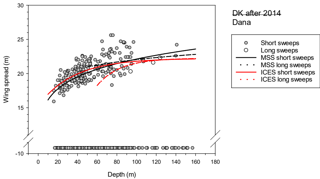
Figure 5.5. DK / RV Dana: Wing spread in relation to depth, Q1 and Q3 (long sweeps were used in 1Q 2015 for the last time).
