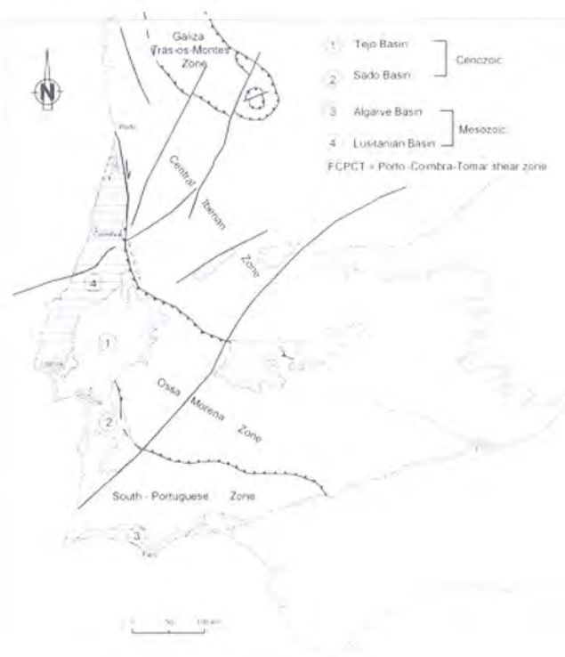
Fig. 1.1 – The geotectonic domains.
