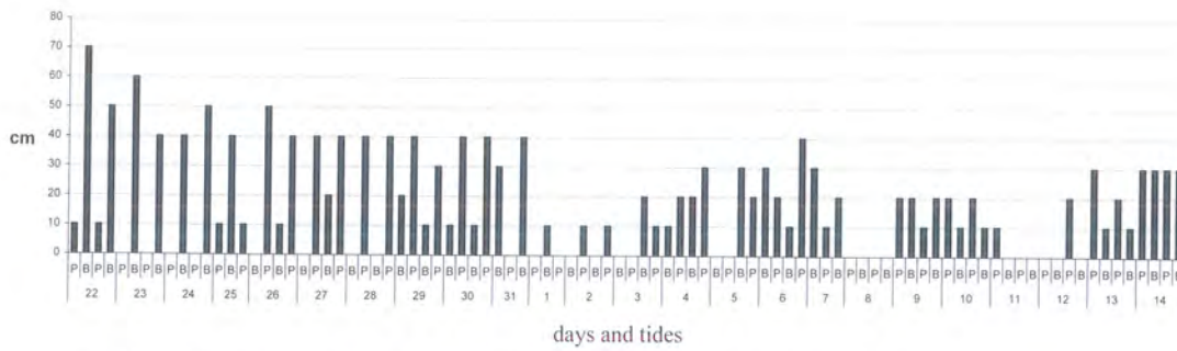
Fig. 9.8 – Storm surge from 22/12/1995 to 14/1/1996. (Pereira et al , 1997).
