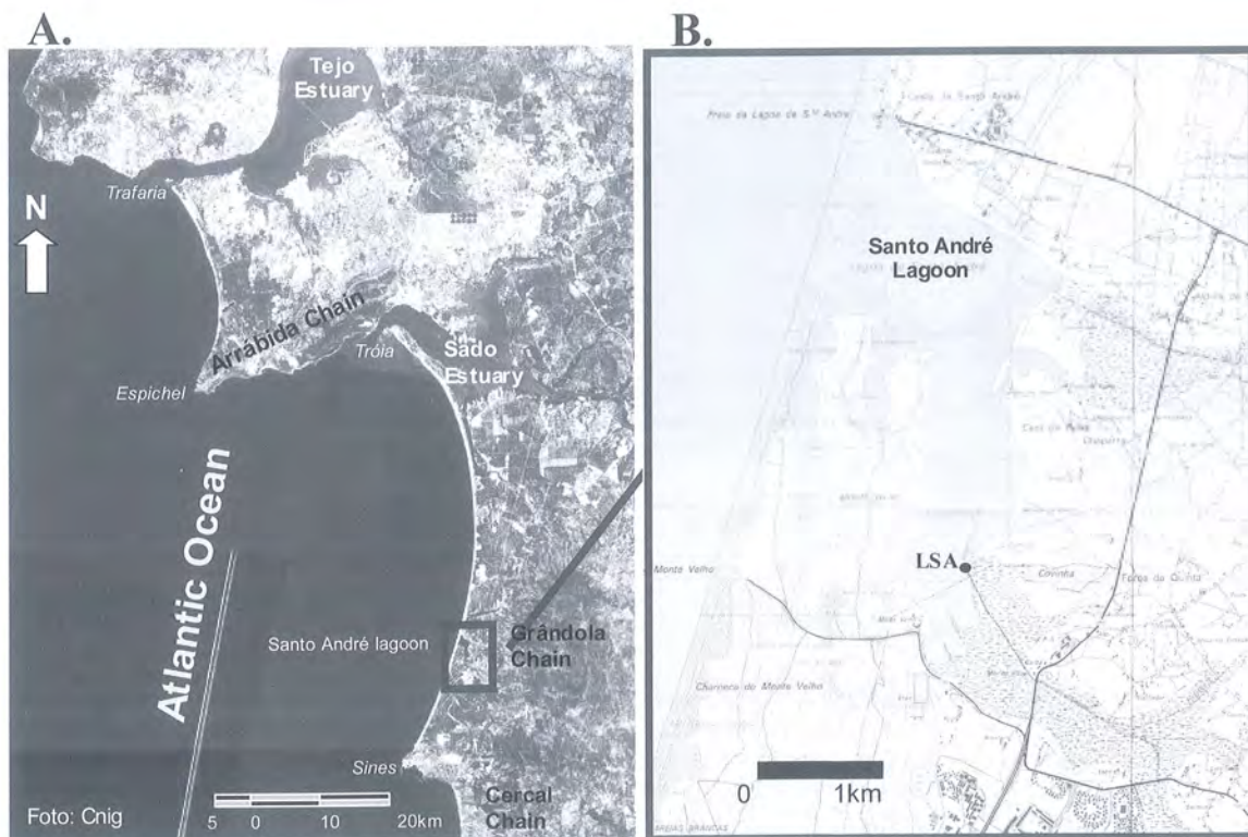
Fig. 10.1 - Location of Santo André lagoon.
