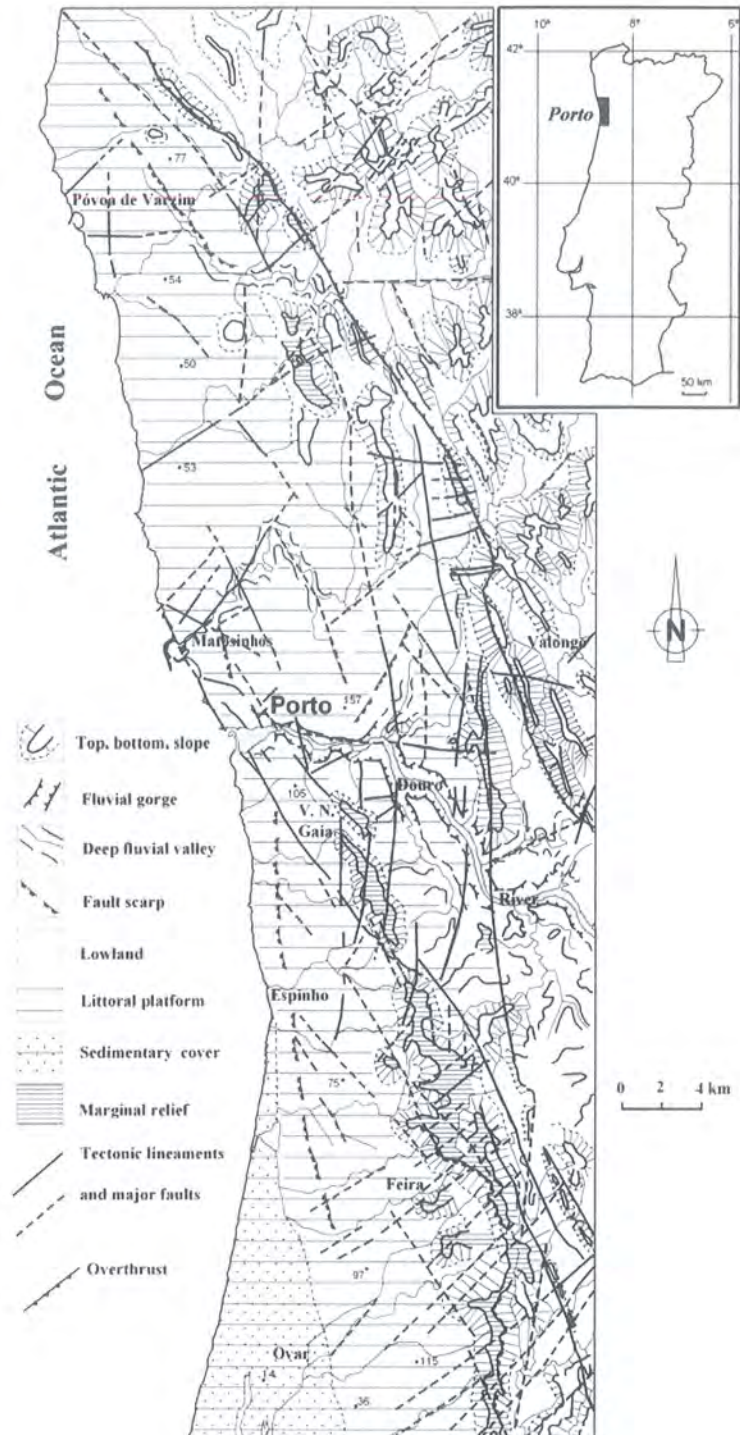
Fig. 2.1 – Geomorphological setting of Oporto region.
