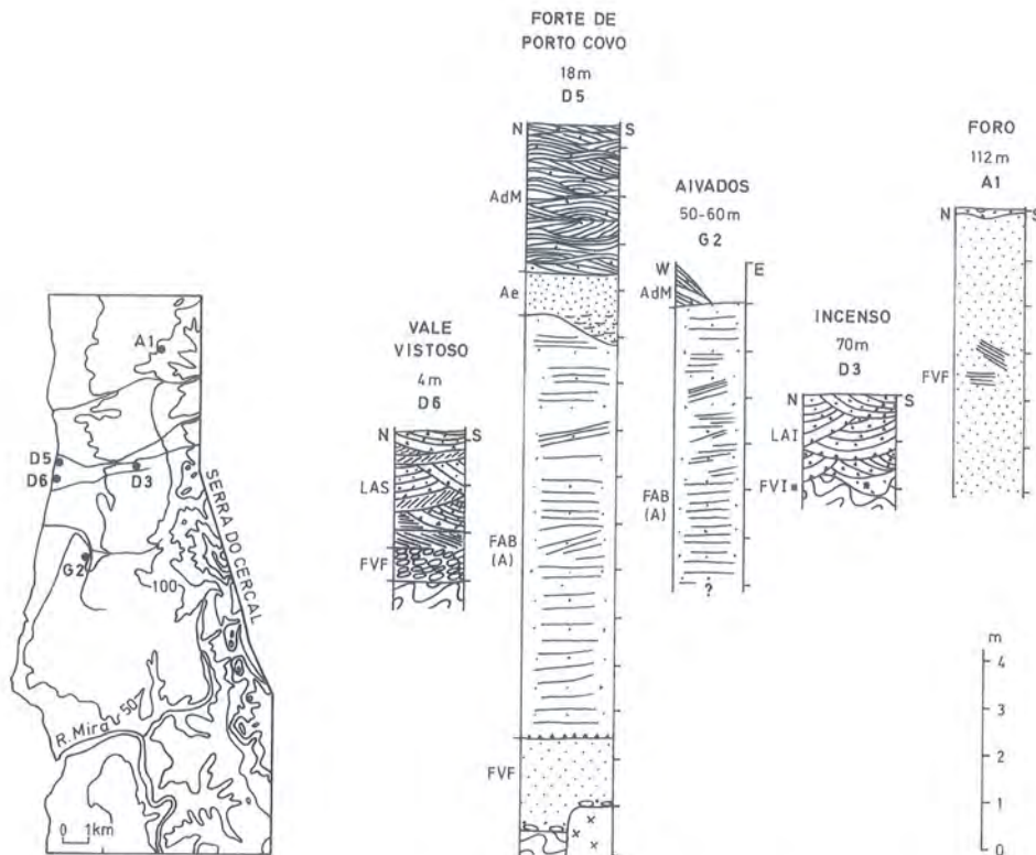
Fig. 11.2 – Logs of the deposits preserved on the littoral platform north of Vila Nova de Milfontes (Pereira, 1990).
