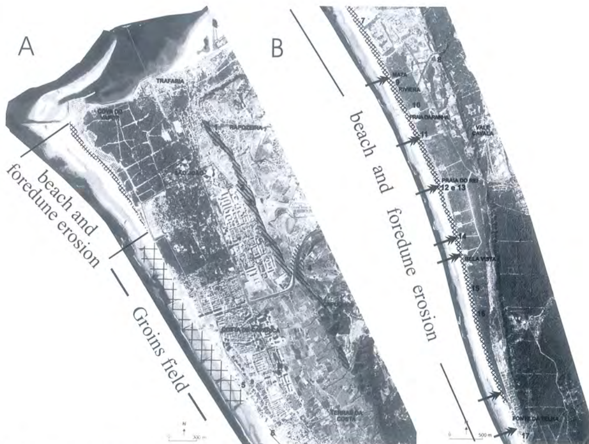
Fig.9.9 – The Northern half of the Caparica arc. The arrows show the overwashes during the December 95-January 96 sea storm event. Adapted from Ferreira, 1999.
