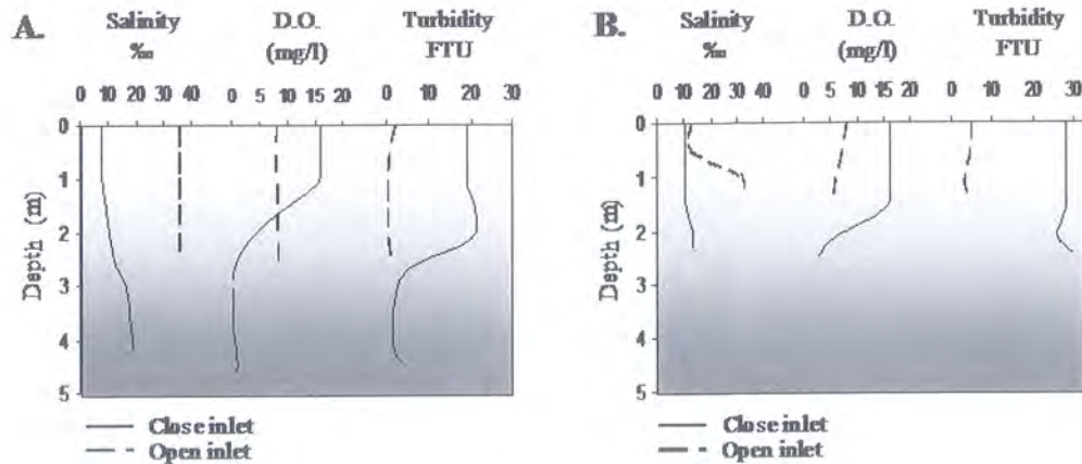
Fig. 10.7 – Vertical profiles of physico-chemical parameters of Santo André lagoon in open and closed inlet periods. A - 1998. B - 1999.
