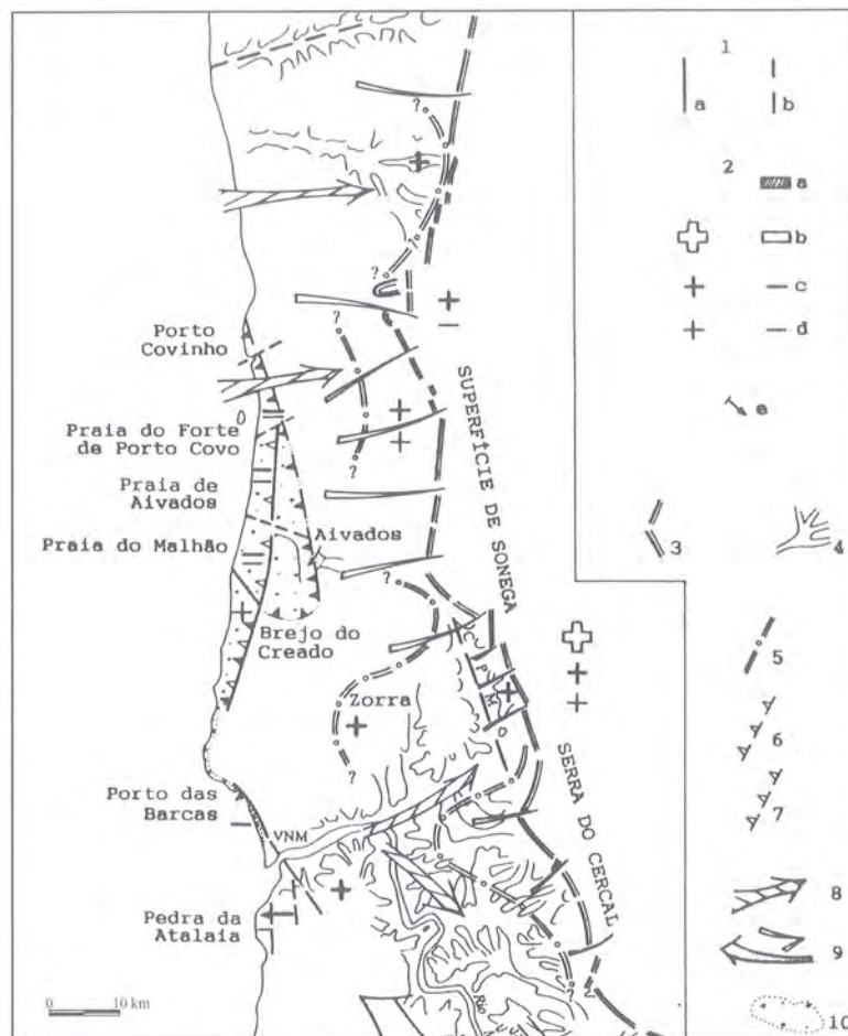
Fig. 11.6 - The polygenic evolution of the littoral platform near Vila Nova de Milfontes. 1- tectonic lineations: a – fault; b – probable fault; 2 – relative displacement of the tectonic compartments: a – previous or locally correlative of Red Formation; b – post Red Formation; c – post Aivados-Bugalheira Formation; d – post Malhão aeolianite and direction of tilting; 3 – scarp slope of Serra do Cercal; 4 – main valleys entrenching the platform; 5 – approximate position of the contemporaneous Red Formation coastline; 6 – correlative cliff of the Aivados-Bugalheira Formation; 7 - correlative cliff of the Monte Figueira Formation; 8 – sea transgression during Red Formation deposition; 9 – alluvial fans advance; 10 – Aivados-Bugalheira Formation extension (Pereira, 1990).
