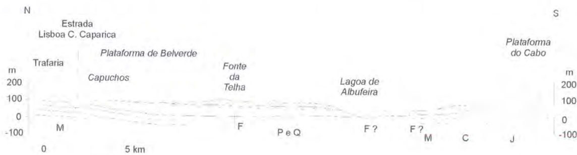
Fig. 9.11 – The structure of the rocks cut in the heritage cliff of Costa da Caparica. J – Jurassic; C – Cretaceous; M – Miocene; P – Pliocene; Q - Quaternary (Pereira, 1988).
