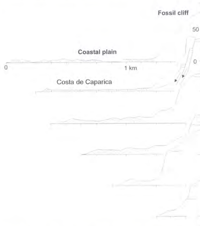
Fig. 9.3 – The coastal plain of Costa da Caparica and the fossil cliff (Pereira, 2003).
