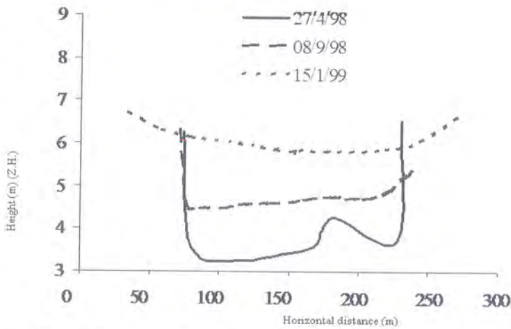
Fig. 10.6 – Major vertical accretion episodes recorded within the scar of the Santo André former inlet.
