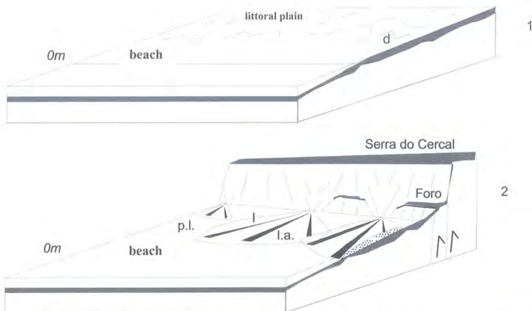
Fig. 11.3 – The evolution of the littoral platform dominated by Serra do Cercal during the Pliocene (1) and the Plio-Quaternary transition (2) (Pereira, 1999). 1 - the littoral plain bathed by the sea, with beach and dunes (d); 2 – littoral gravel plain (p.l.), with alluvial fans (l.a.), bathed by the sea and dominated by Serra do Cercal (legend in fig. 11.5).
