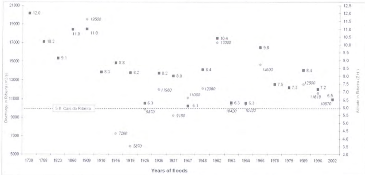
Fig. 3.4 – Extraordinary floods in Ribeira – Porto (IHRH, 2003). The altitudes are referred to hydrographic zero (1,8m under topographic zero).
