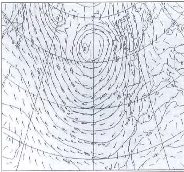
Fig. 9.6 - Synoptic chart of the 6 January 1996. Daily bulletin of the Meteorological National Institute
