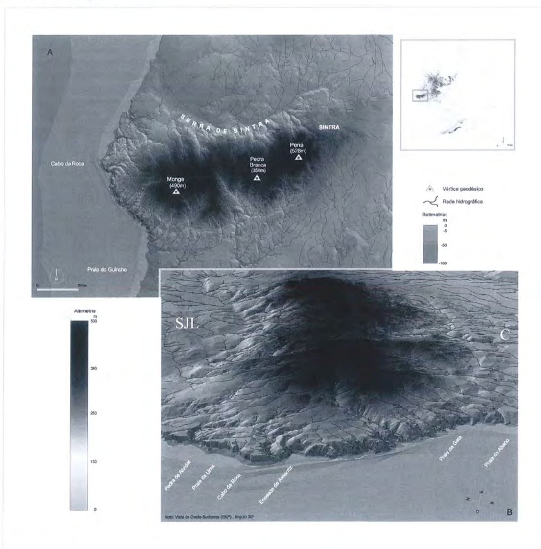
Fig.8.1 – Serra the Sintra and S. João das Lampas (SJL) and Cascais (C) elements of the littoral plataform. From Pereira, 2003.
