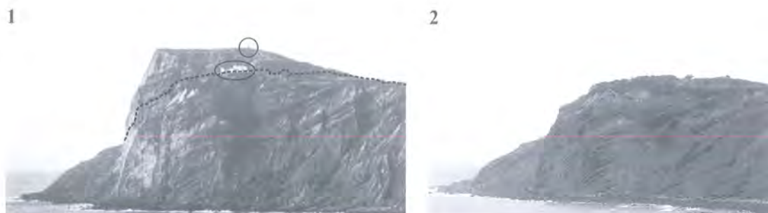
Fig. 6.2 – Ponta do Facho in: 1–1952/53 (©Foto Beleza); 2–September 2003 (©MNeves). In photo 1, the dashed line indicates the present topography, the circle identifies the geodesic landmark of Facho 2'' and the ellipse points out the position of the Facho Café .
