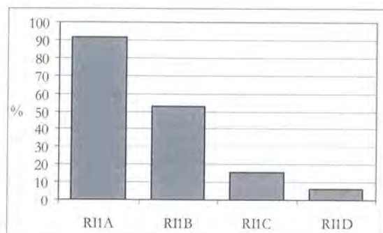
Fig. 7.2 - Annual submersion period for each TMEM measurement Areas at Ribeira de Ilhas (in %).
