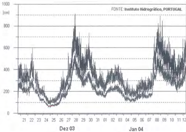
Fig. 3.2 – An example of significant and maximum wave high during a storm period at Leixões buoy (www.hidrográfico.pt).
