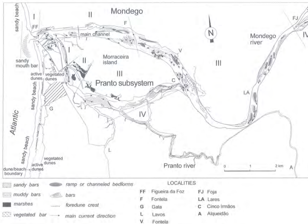
Fig. 5.7 – Longitudinal geomorphological zonation of the Mondego and Pranto estuarine subsystems in 1947, comprising four major segments (authors: German Flor & P.P. Cunha; Cunha et al , in press): I) Mouth Complex; II) Sandy Bay; II) Mudflats; and IV) Upper Channel. Arrows show the main currents deduced in the spillover lobes, responsible for the sediment distribution by tidal or fluvial flows. The Mondego subsystem is dominated by fluvial discharge, while the Pranto subsystem is tide dominated.
