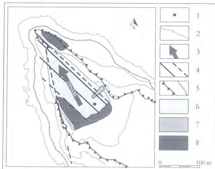
Fig. 6.5 – Geomorphological sketch of Ponta do Facho.
