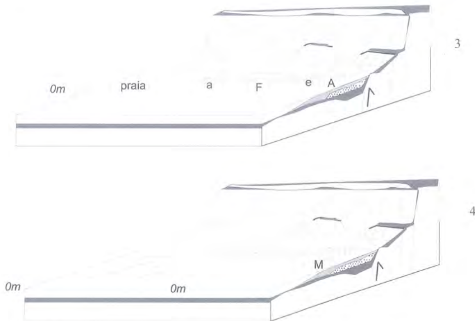
Fig. 11.4 - The evolution of the littoral platform dominated by Serra do Cercal during the Lower and Middle Pliocene (?). 3 - e - scarp fault, a - cliff cut into the alluvial fans, A - Aivados, F - Fort). 4 - littoral platform covered by a large dune field (M - Malhão), after a sea retreat. (Pereira, 2000). (Legend in fig. 11.5).
