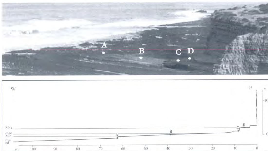
Fig. 7.3 – Localization of the 4 TMEM measurement Areas in the Ribeira de Ilhas shore platform: above —on a photo taken the 17/04/03 (tide at 0,3m a.c.d); below —on the Ribeira de Ilhas topographic profile, with reference to the tide levels. Mhs —Maximum high water spring level; mhn —minimum high water neap level; Min —Maximum low water neap level; mls —minimum low water spring level; cd —chart datum.
