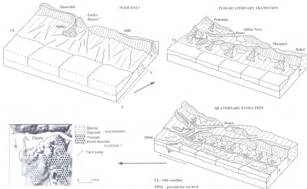
Fig. 2.3 – Geomorphological evolution of Porto littoral platform (Araújo et al. , 2003).
