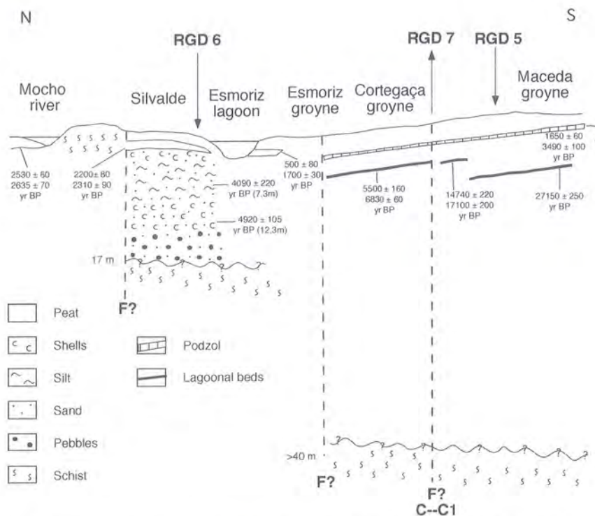
Fig. 4.2 – Schematic cross-section along the coast showing the Esmoriz lagoon emplacement.
