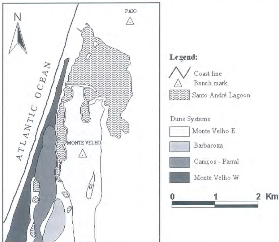
Fig. 10.3 – Present-day beach-foredune system cutting older ridge and slack and relation with Santo André lagoon.
