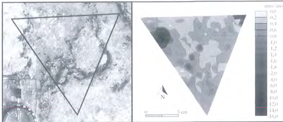
Fig. 7.7 – On the left, RIIC measurement Area on 30 June 2003. On the right, RIIC annual downwearing rate registered in winter 2002/03 (period 4-5).
