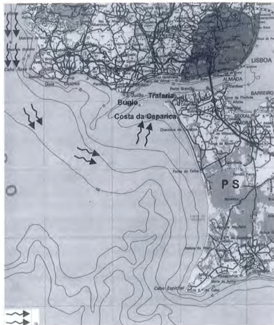
Fig.9.1 – The western littoral of Setúbal Peninsula. a – longshore drift.
