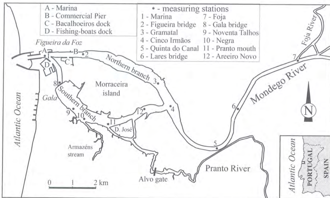
Fig. 5.5 – Mondego estuary (except a small portion of the upstream sector) (Cunha e Dinis, 2002).
