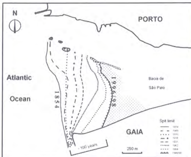
Fig. 3.3 – The retreat of the sand spit since 1854 to 1996-98. Administração do Porto Douro – Leixões (1999).
