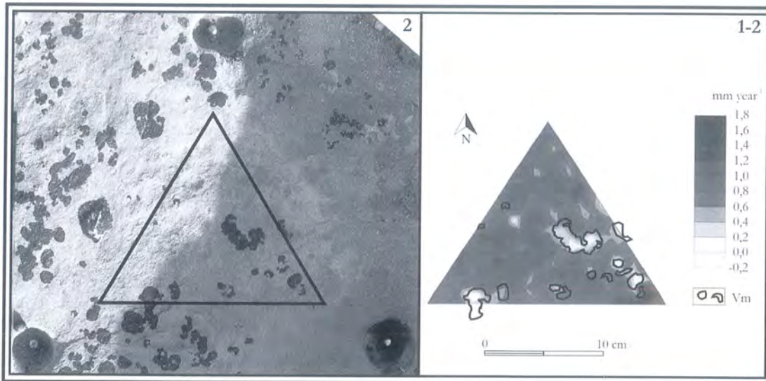
Fig. 7.6 – Influence of the Verrucaria maura (Vm) distribution area in the swelling results (measurement 1-2 – summer 2001).
