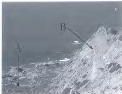
Fig. 6.3 – Failure surfaces of 1954 Ponta do Facho landslide. A – marl-clay layer; B – fault with azimuth N132°. Photos taken in September 2003.
