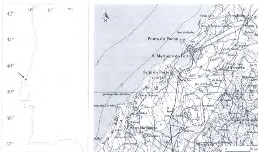
Fig. 6.1 – Localization of Ponta do Facho-Praia da Gralha studied area.
