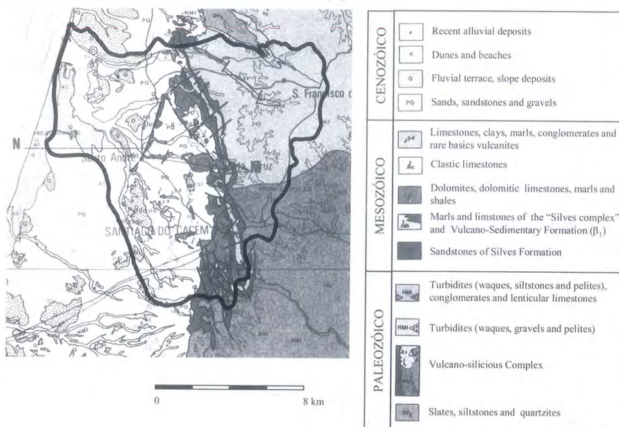
Fig. 10.2 – Geological setting of Santo André lagoon watershed.
