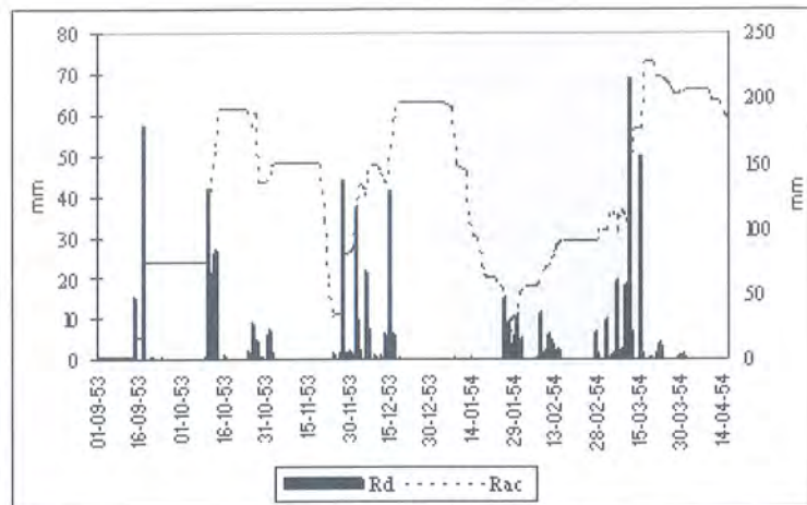
Fig. 6.4 – Rainfall, daily (Rd) and accumulated for forty days (Rac), at Alfeizerão between September 1, 1953 and April 15, 1954. The shadowed area indicates the activity period of the 1954 Ponta do Facho landslide.
