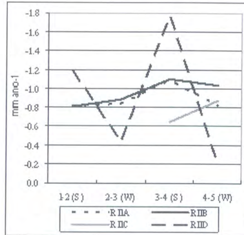
Fig. 7.5 – Annual average downwearing rates for Ribeira de Ilhas TMEM Areas in each measurement period: S-summer; W-winter.
