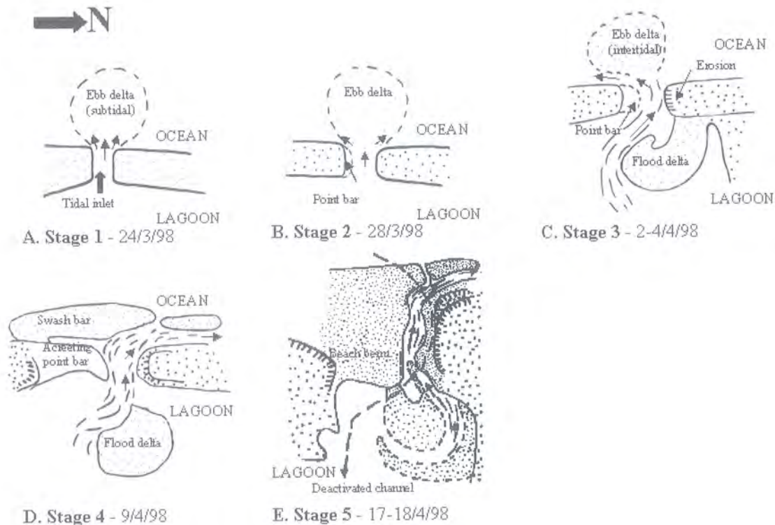
Fig. 10.5 – Schematic stage model of inlet morphodynamic changes.
