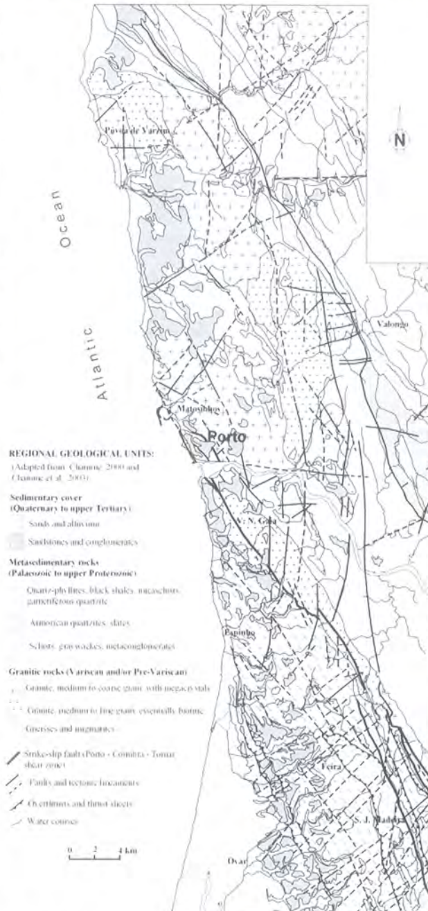
Fig. 2.2 – Geological framework of Porto region.
