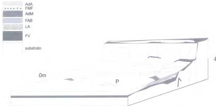
Fig. 11.5 - Present day landscape (P – Pessegueiro Island). Deposits from the oldest to the youngest: FV – Red Formation (FVF); LA – alluvial fan; FAB – Aivados-Bugalheira Formation; AdM – Malhão aeolianite; AdA– Aivados aeolinite (Pereira, 1999).
