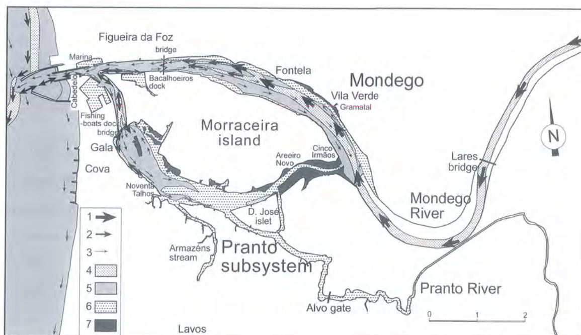
Fig. 5.8 – Grain-size distribution and sediment circulation scheme in the Mondego estuary and adjacent beaches (Cunha & Dinis, 2002): maximal transport capability of traction currents (1 - up to granules, 2 - up to very coarse sands, 3 - up to medium sands); superficial sediments mean grain-size (4 - granules to coarse sand, 5 - medium to fine sand); tidal mudflats, muddy and channel bottoms (6); salt marshes (7).
