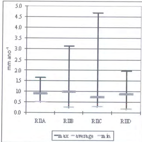
Fig. 7.4 – Annual downwearing rates for Ribeira de Ilhas TMEM Areas: absolute maximum (max), average and absolute minimum (min).
