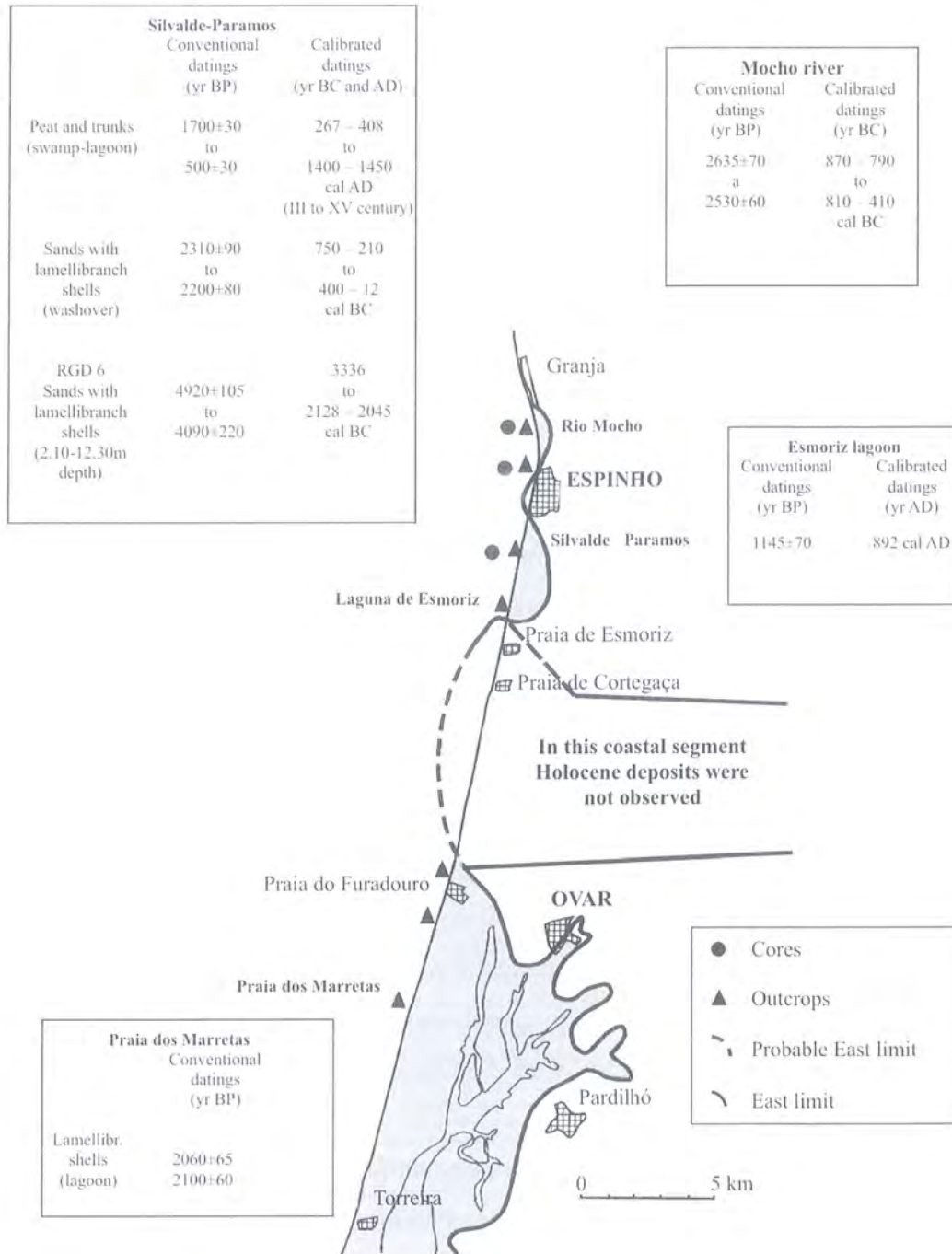
Fig. 4.1 – Probable limits of the Holocene lagoon system between Espinho and Torreira, including the Ovar barrier of the present Aveiro lagoon.
