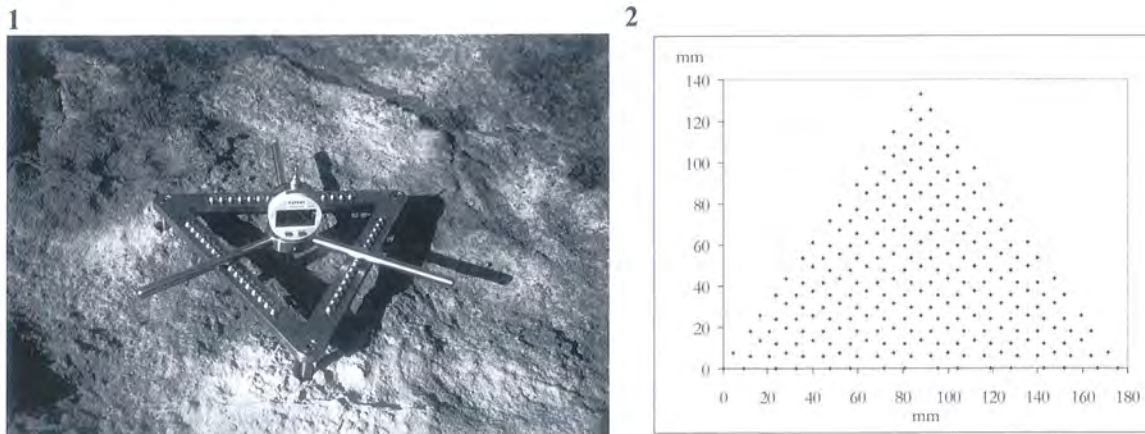
Fig. 7.1 – 1-TMEM installed in one of the studied areas; 2-Relative position of the 255 points measured by the TMEM.
